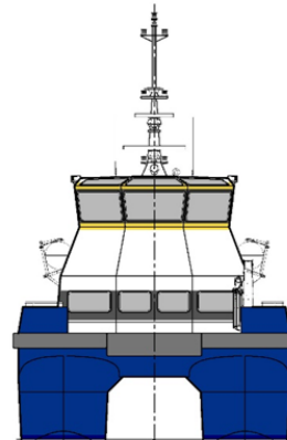
VIEW ON BOW
